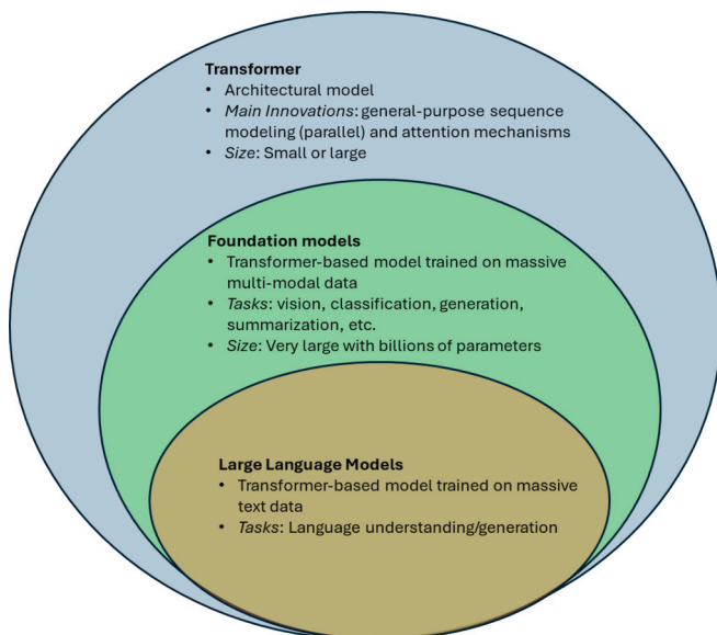
Fig. 1. Hierarchical taxonomy of types of models described in this work.
