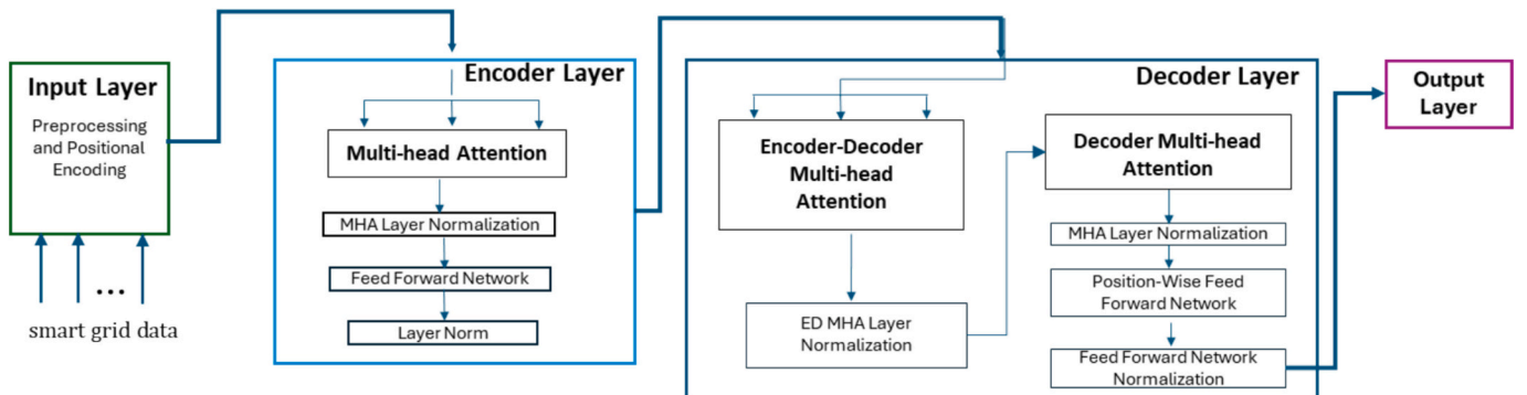
Fig. 2. Vanilla transformer for predictive tasks in smart grids.
