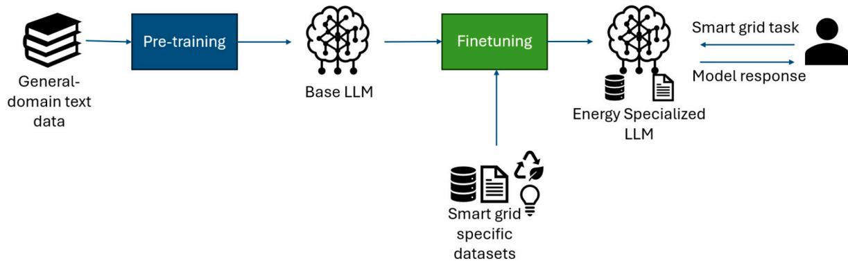
Fig. 3. Finetuning process for LLMs adaptation to smart grid management tasks.
